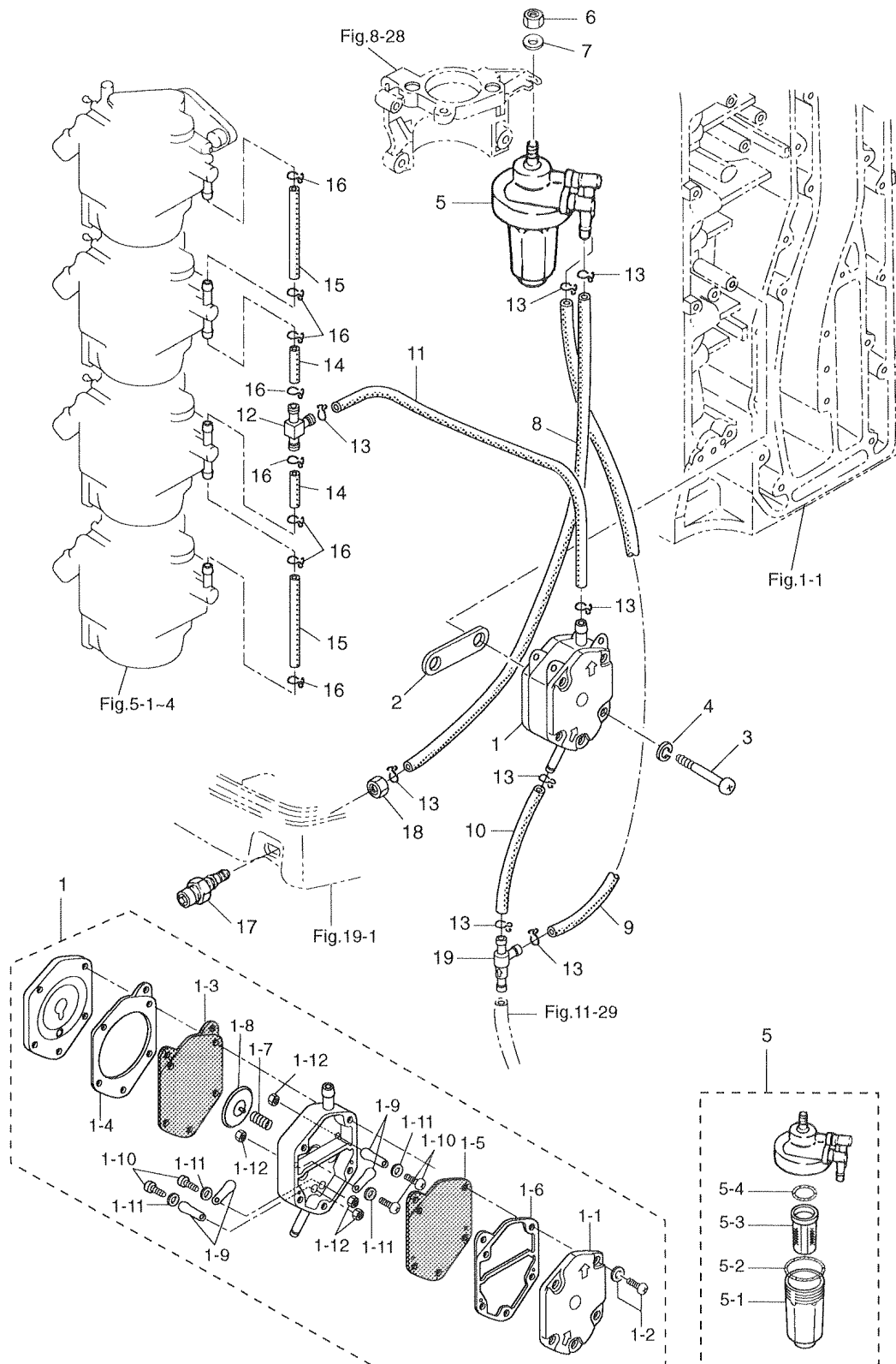
Fig. 6 FUEL PUMP
