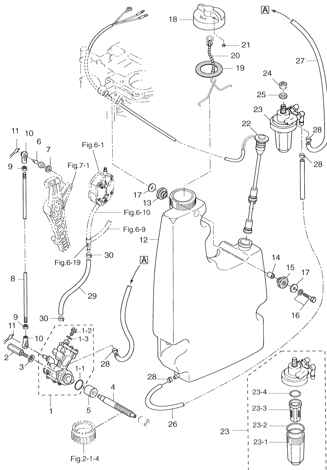
Fig. 11 OIL PUMP
