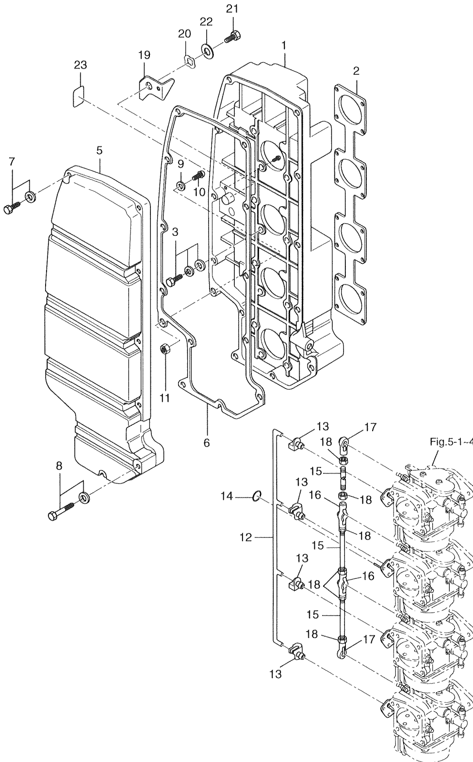
Fig. 4 AIR SILENCER
